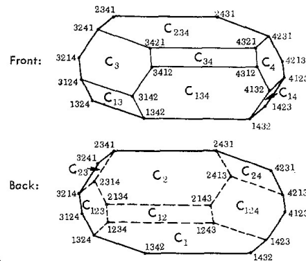
Fig. 2: Core of a four-person convex game
