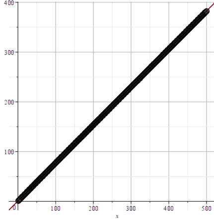
Figure 2: Average of maximum component size over all maps.
