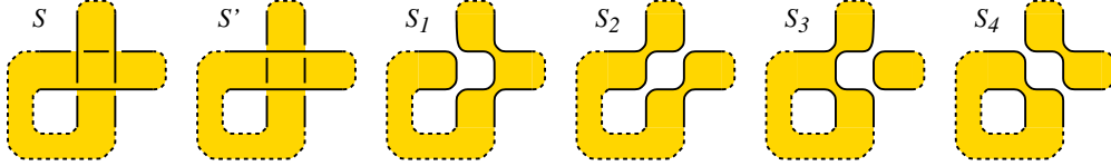
Figure 6: Resolving a pure ribbon singularity
