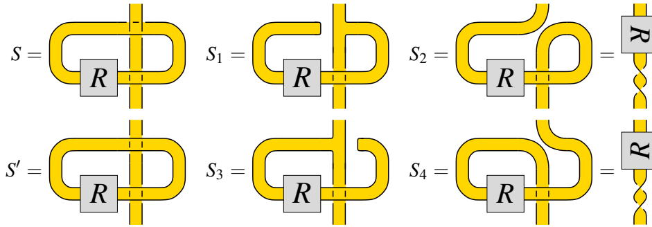
Figure 7: Resolving the only ribbon singularity between S_{=} and S_{\parallel}
