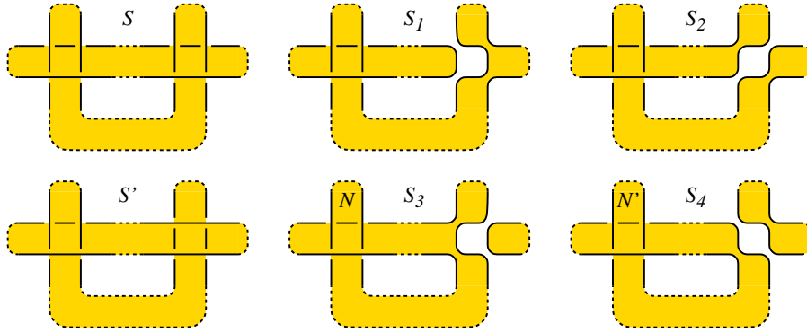
Figure 8: Resolving a second ribbon singularity between S_{=} and S_{\parallel}
