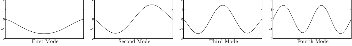
Figure 6.4. First four modes of \tilde{g}
