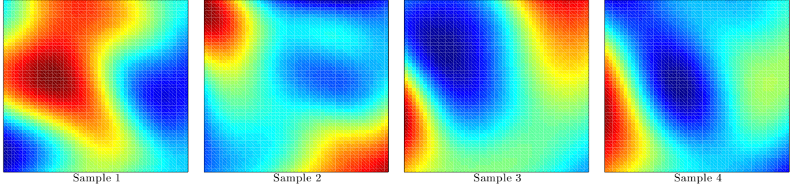
Figure 6.1. Four random realizations of \kappa
