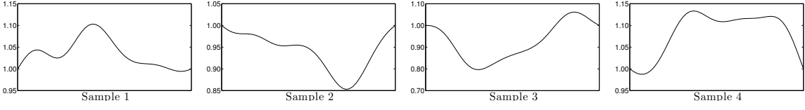
Figure 6.3. Four random realizations of g
