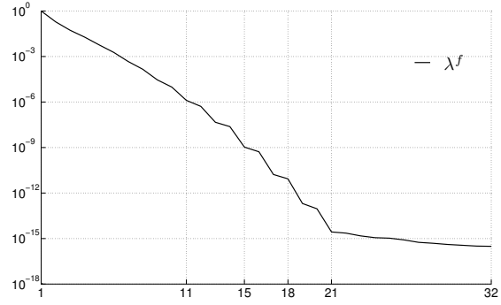
(b) Eigenvalues of the KL expansion of \tilde{g} and KL truncation values K^f = 11 , K_{\max}^f = 15 and K_{\text{detail}}^f = 18
