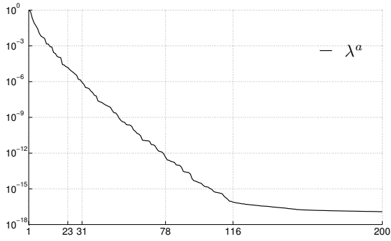
(a) Eigenvalues of the KL expansion of \tilde{\kappa} and KL truncation values K^a = 23 , K_{\max}^a = 31 and K_{\text{detail}}^a = 78
