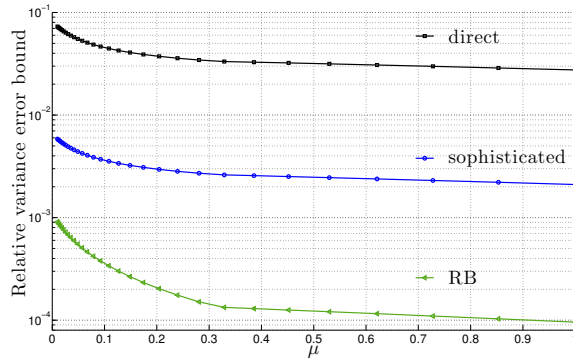
Figure 6.9. Different relative error bounds for variance \mathbb{V}(\mu)
