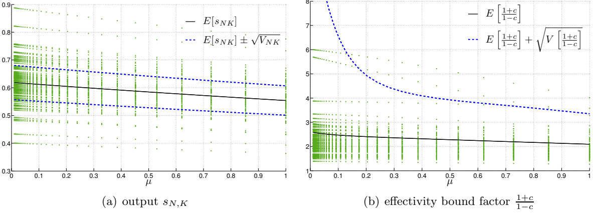
Figure 6.7. Means of output s_{N,K} and of effectivity bound factor \frac{1+c}{1-c} , their standard deviations, and 100 random samples for a test set of 30 logarithmically distributed values of \mu , respectively
