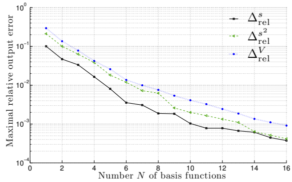
(b) Relative error decay of outputs s , s^2 and \mathbb{V} without \delta_{\text{KL}} -contributions, respectively
