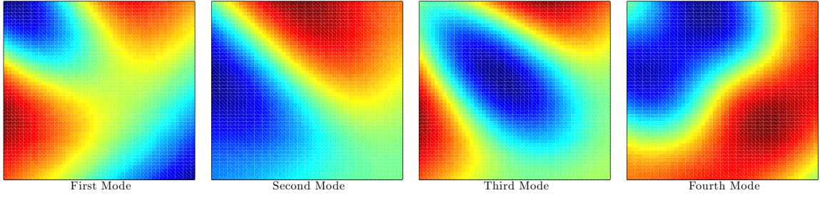
Figure 6.2. First four modes of \tilde{\kappa}
