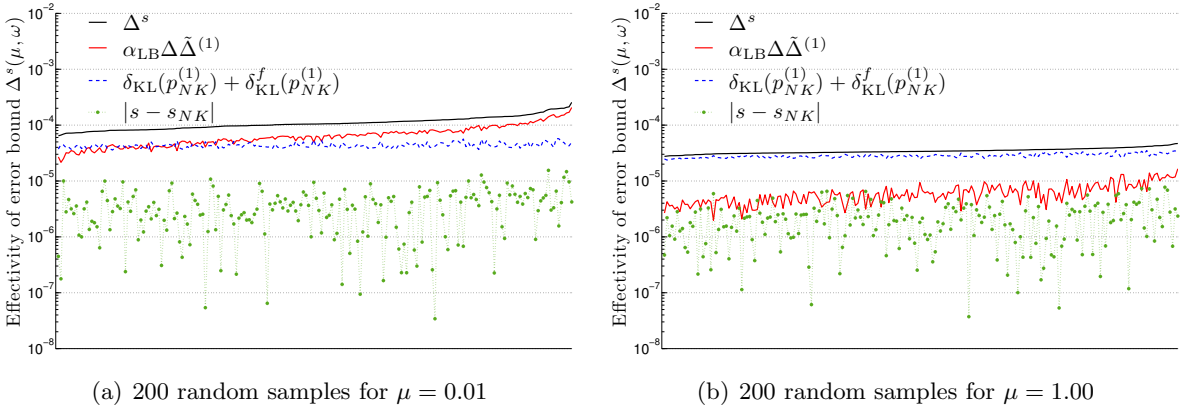
Figure 6.8. Error bound \Delta^s , splitted in its \delta_{KL} - and \Delta -part, and actual output error for 200 random samples and two values of \mu
