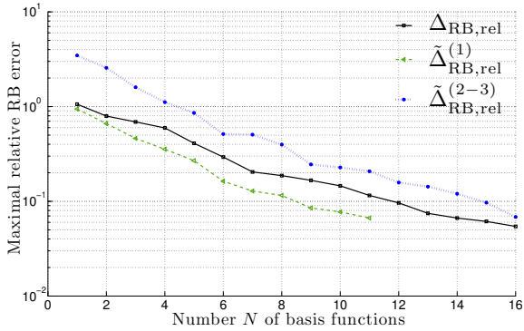
(a) Relative error decay of primal solution u and dual solution p^{(1)} , and of p^{(2)} - p^{(3)}
