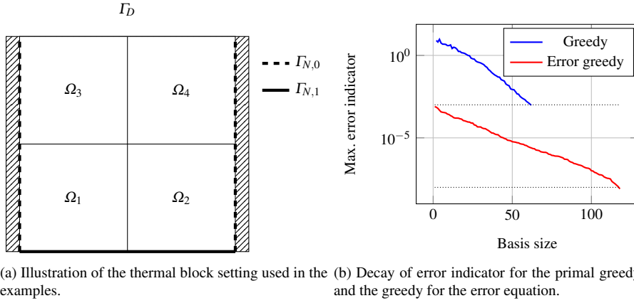
Fig. 1: Test 1: Setting for the thermal block model, decay of error indicator.
