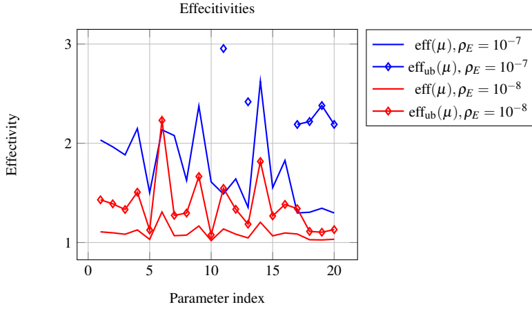
Fig. 3: Test 1: Effectivity of the L^2(\Omega) -norm error bound for 20 random test parameters.
