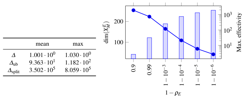
(a) Mean and maximum effectivity for (b) Dimension of the subspace X_M^E (bars) and maximum error bounds for the ARE. effectivity (line) for varying \rho_E .
