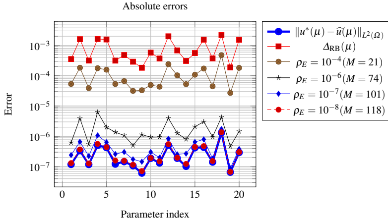
Fig. 2: Test 1: Absolute error measured in the L^2(\Omega) -norm for 20 random test parameters.
